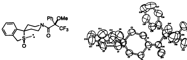
X-ray ORTEP of ( R )-MTPA amide of ( S )- 1
